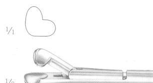
SCHEINMANN DF-425-4984 for interchangeable tubes DF-425-4977 - DF-425-4980
