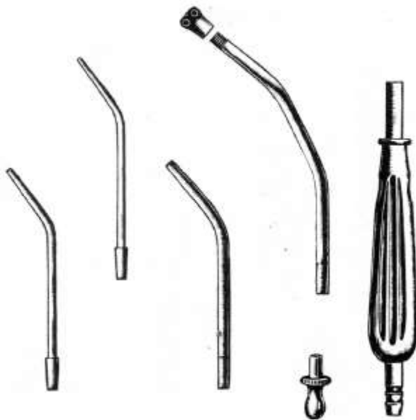
DF-161-1862 + DF-161-1863+1864+1865+1866+1867 Yankauer Suction Tube Set (31cm) Complete Set with connectors and suction tip
